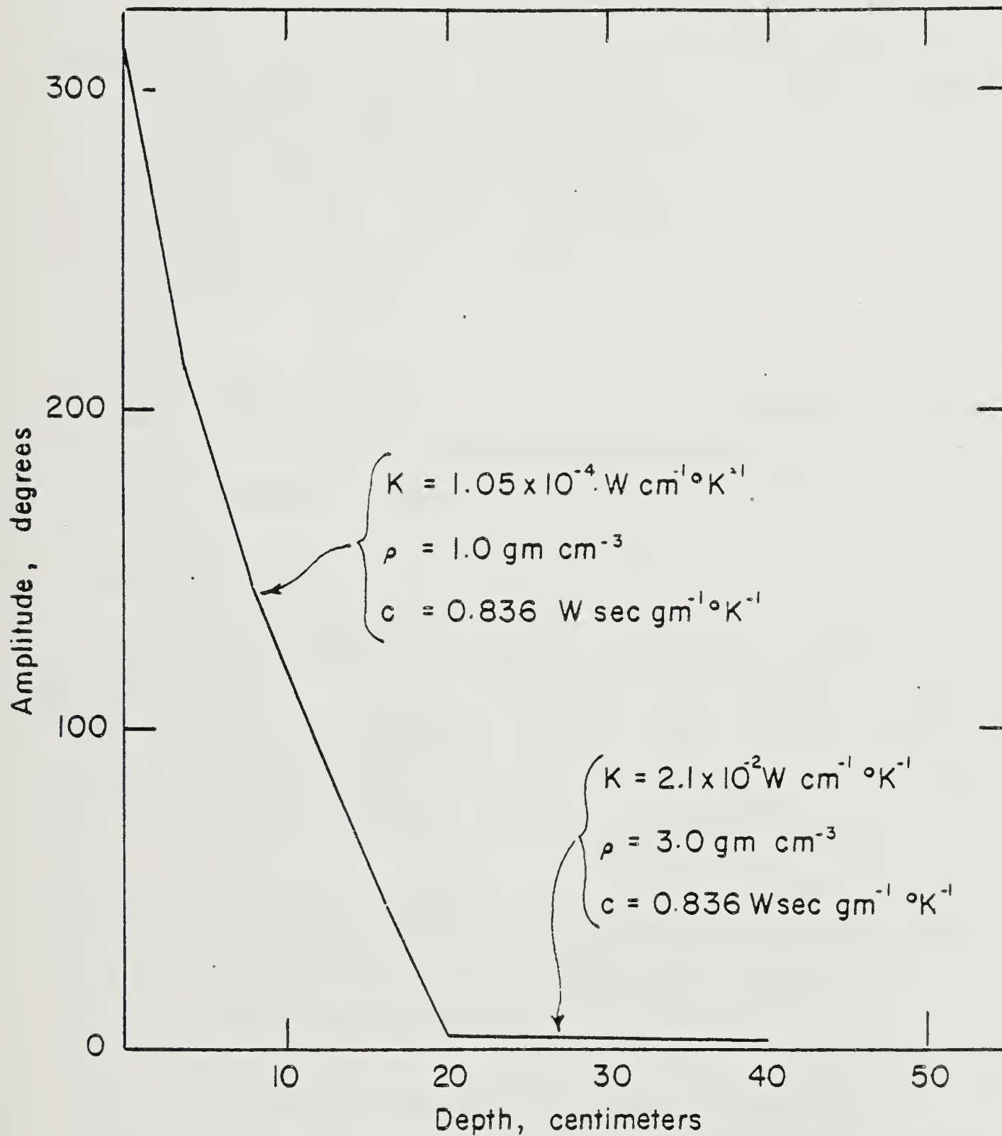
Effect of properties of the surface material on amplitudes.
